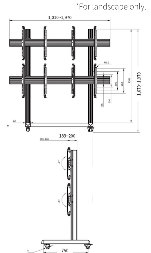
2x2 Multi-monitor Floor stand FS2B2 (supplied by Eagle Mount)
